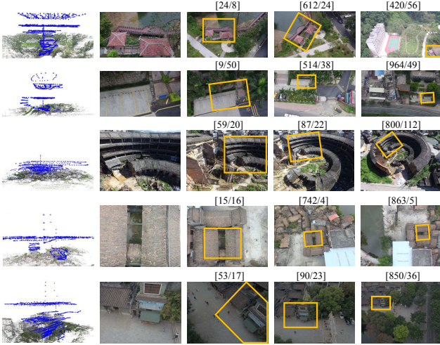
Figure 5: Our multi-scale retrieval dataset including 5 scenes. In each row, camera poses are first displayed, then one of the 5 queries in each scene followed by 3 sample database images at different scales. Common areas shared with the query are marked by yellow bounding boxes. The two numbers in square brackets above each image are the ranks given by the baseline [31] and baseline+our similarity metric respectively.
