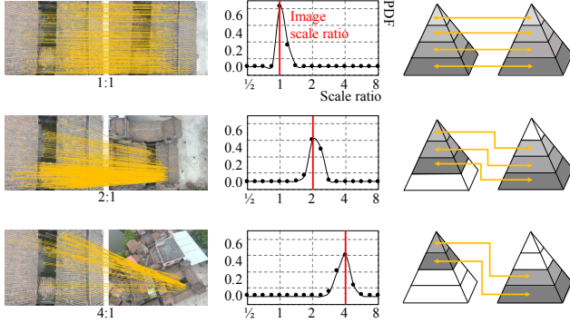
Figure 2: Illustration of three match pairs with image scale ratio around 1, 2, and 4. The left column visualizes the feature matches. The middle column is the PDF of scale ratios of the inlier feature matches. Following the scale consistency [13, 19], the scale ratios are quite centralized. Deduced from the scale consistency, inlier correspondences are supposed to link between the scale levels in scale space with consistent discrepancy as shown in the right column.
