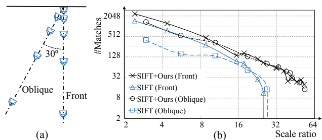
Figure 7: (a) Capture pattern of book-cover image set. (b) Number of correct matches with regard to image scale ratio in logarithm scale achieved by SIFT matcher and ours. SIFT matching fails when the image scale ratio exceeds 25 while our methods shows its superiority in both match number and robustness to scale variations even when the image scale ratio approaches 60.
