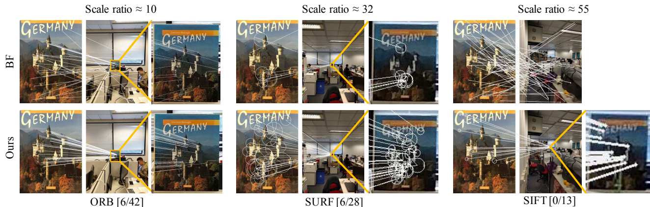
Figure 6: Visualization of matching results using ORB [35], SURF [3] and SIFT [23] features by brute-force (BF) matcher and our scale-invariant matcher. The two numbers in below square brackets denote the correct match numbers achieved by two methods respectively.
