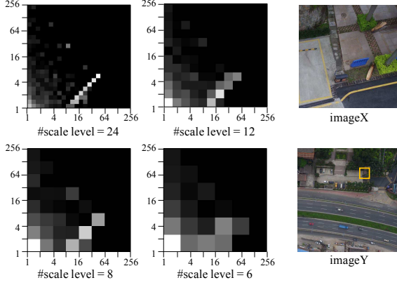
Figure 3: Scale level matching maps of images X and Y in the right column with scale ratio around 10. The overlap region is marked in yellow box. The scale range of 1 to 256 is divided into different numbers of scale levels. The higher brightness of each square reflects the stronger matching response between corresponding scale levels. Following the scale consistency deduction in Equation 5, line patterns in anti-diagonal direction are observed indicating constant discrepancy between related scale levels.
