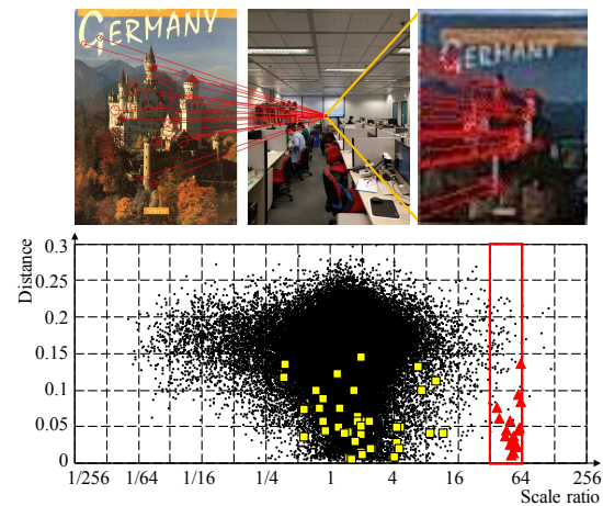
Figure 1: The top row visualizes the SIFT matches found by our approach between images holding scale ratio around 55. The black dots in below chart represent 69640 putative matches, characterized by feature scale ratio and descriptor distance. The yellow squares denotes the false positive correspondences found by modern SIFT match strategies [23, 46, 43, 9]. Conversely, our approach first determines the related scale levels in scale space that enclose the feature correspondences. Then image matching is restricted between the related scale levels. The red box encloses the 90 feature pairs existing between related scale levels, including 20 inlier correspondences found eventually denoted by red triangles.
