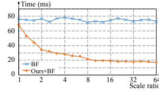
Figure 4: Time of pairwise matching with respect to the image scale ratio between around 50k \times 50k SIFT sets implemented by GPU. Our approach keeps on improving the efficiency of brute-force (BF) search as the scale ratio increases.
